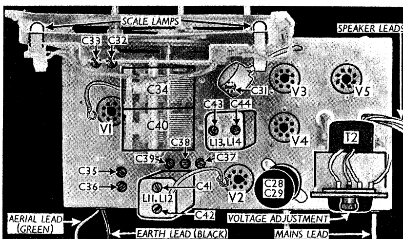
Plan view of the chassis. The positions of the tuning drive drum and the pointer, with the scale backing plate between them can be seen here.
