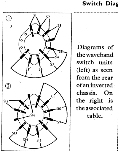
Switch Diagrams and Table.
